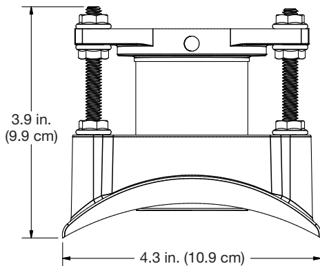
SADDLE - FRONT VIEW
